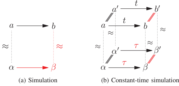
Fig. 4: Lockstep simulations
