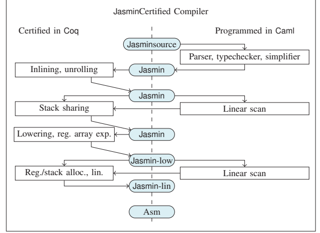
Fig. 12: Jasmin architecture [4].
