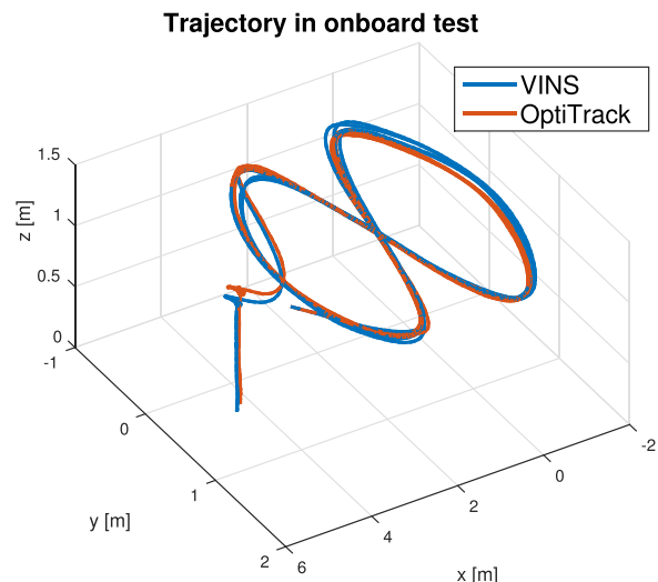
Fig. 22. Trajectory of loop-closure-disabled VINS-Mono on the MAV platform and its comparison against the ground truth. The robot follows the trajectory four times. VINS-Mono estimates are used as the real-time position feedback for the controller. Ground truth is obtained using OptiTrack. Total length is 61.97 m. Final drift is 0.18 m.
