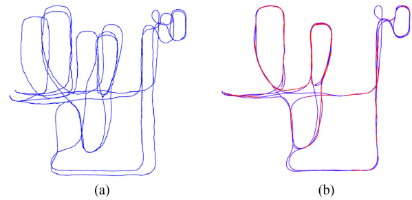
Fig. 19. Results of the indoor experiment with comparison against OKVIS. (a) Trajectory of OKVIS. (b) Trajectory of the proposed system. Red lines indicate loop detection.
