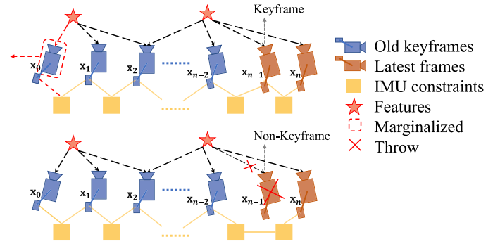
Fig. 7. Illustration of our marginalization strategy. If the second latest frame is a keyframe, we will keep it in the window, and marginalize the oldest frame and its corresponding visual and inertial measurements. Marginalized measurements are turned into a prior. If the second latest frame is not a keyframe, we will simply remove the frame and all its corresponding visual measurements. However, preintegrated inertial measurements are kept for nonkeyframes, and the preintegration process is continued toward the next frame.
