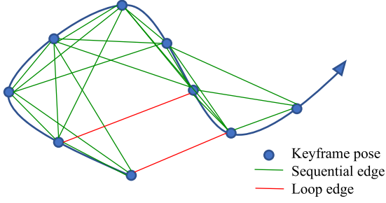
Fig. 12. Illustration of the pose graph. The keyframe serves as a vertex in the pose graph and it connects other vertexes by sequential edges and loop edges. Every edge represents relative translation and relative yaw.
