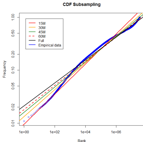
Fig. 1: Yahoo! CDF-Zipf Subsampling
