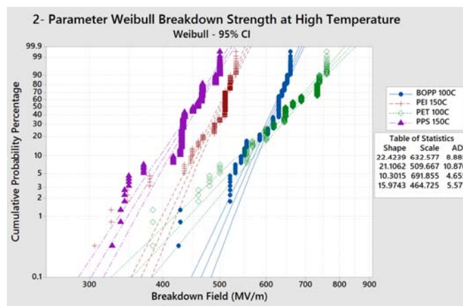
Figure 10. High temperature ASTM D-149 breakdown strength of various polymer films.
