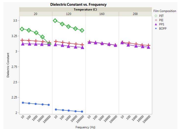
Figure 6. Dielectric constant as a function of frequency and polymer film type at 20°C.
