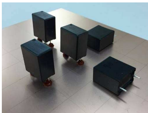
Figure 4. Reflow solder test capacitor orientation.
