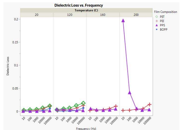
Figure 7. Dielectric loss (loss tangent) as a function of frequency and polymer film type at 20°C through 200°C zoomed out to show low frequency loss of PPS.
