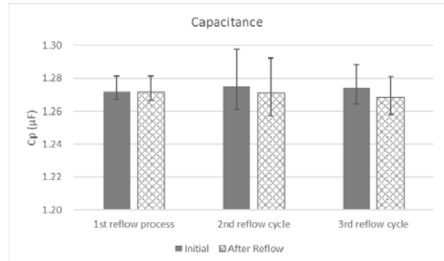
Figure 13. Capacitance change before and after reflow soldering.
