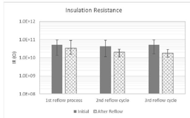
Figure 14. Insulation resistance change before and after the reflow process.
