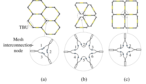
Fig. 4. Reconfigurable Mesh designs (upper): (a) Hexagonal type [23], (b) triangular type [23], (c) square type [26], and their associated interconnections points (bottom).
