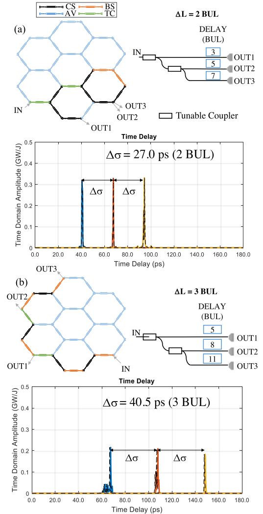
Fig. 12. Layouts and measured performance for two optical beamformer networks with different incremental delay implemented with the 7 hexagonal waveguide mesh: (a) 2-BUL delay, (b) 3-BUL delay.
