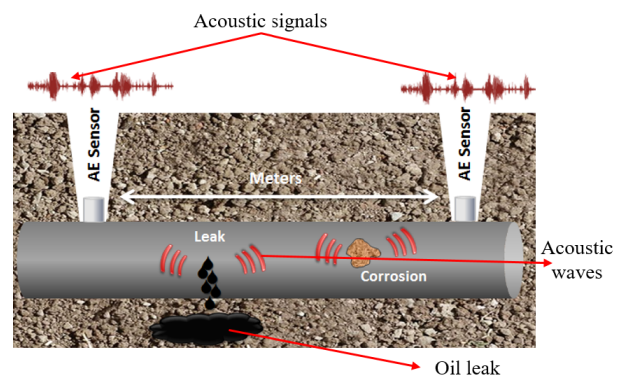
FIGURE 2. Acoustic emission method for pipe leakage detection [21].
