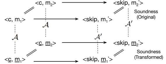
Figure 12: Soundness of original and transformed programs.
