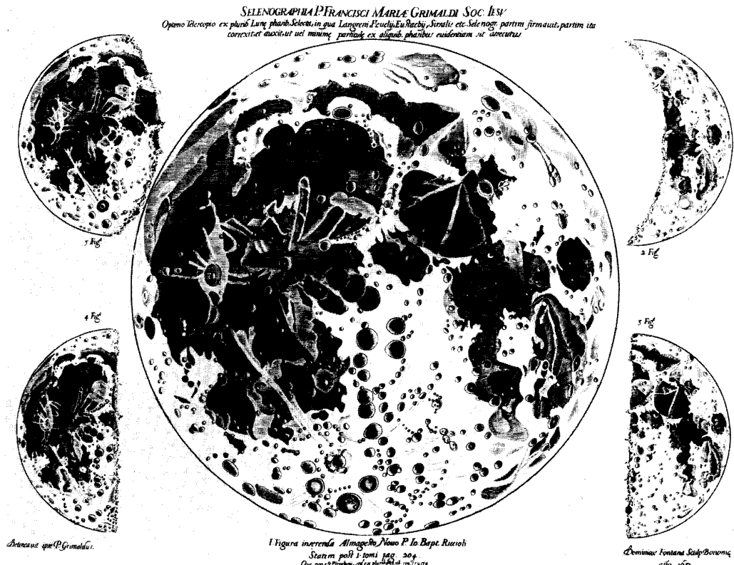
Figure 3. Selenograph of the Moon.
