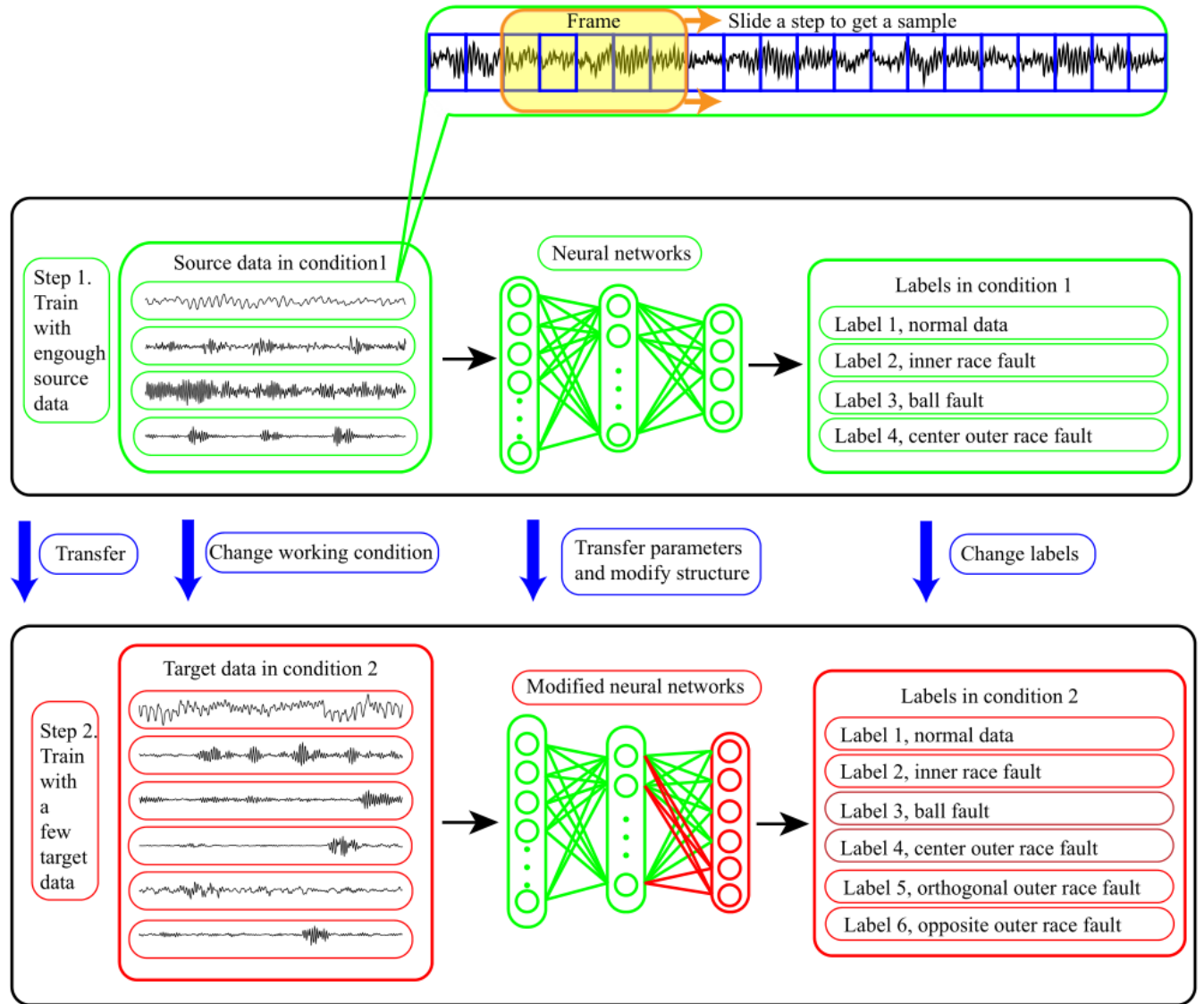
FIGURE 1. Transfer learning based fault diagnosis model.
