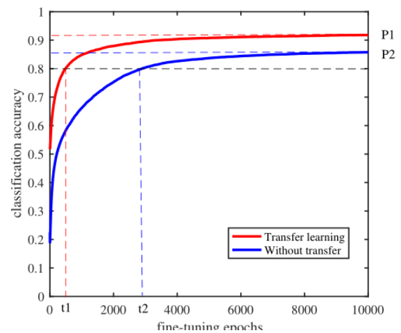
FIGURE 5. Total testing data classification accuracies of different methods. The horizontal axis represents the fine-tuning time in training process and the vertical axis is the classification accuracy.
