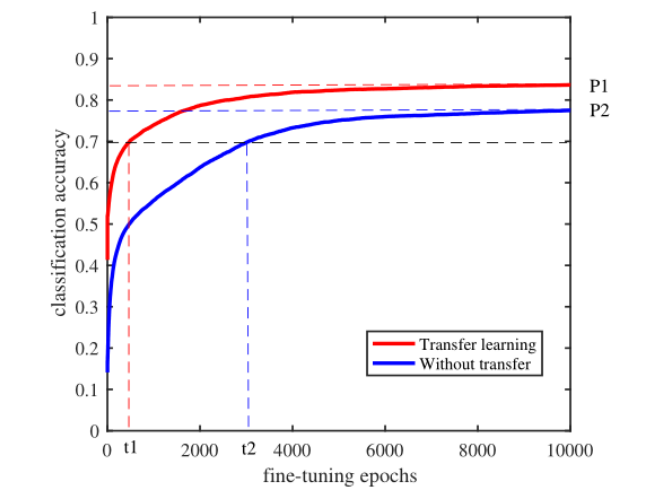
FIGURE 8. Total testing data classification accuracies of different methods. The red line represents the performance of transfer learning method which transfers from working condition 1 to working condition 3. The blue line is the performance of neural networks method without transfer learning. The horizontal axis represents the fine-tuning epochs in training process and the vertical axis is the classification accuracy.
