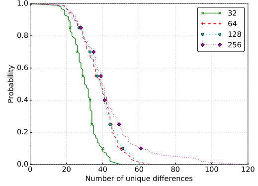
Fig. 10: Probability of finding at least n unique discrepancies across OpenSSL, LibreSSL, and BoringSSL with NEZHA running under output \delta -diversity, for varying numbers of error codes, after 100,000 executions (average of 100 runs, starting from a different seed corpus of 1000 certificates in each run).
