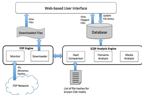
Fig. 1. Overview of the iCOP toolkit
