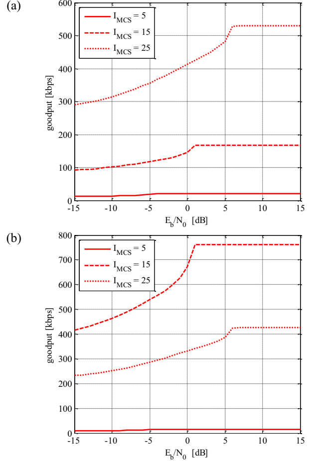
Figure 7. Influence of the radio channel condition ( E_b/N_0 ) on the hidden channel capacity for 1 500-byte IP packets as a function of the MCS used and available resources – (a) N_{RB} = 20 and (b) N_{RB} = 70
