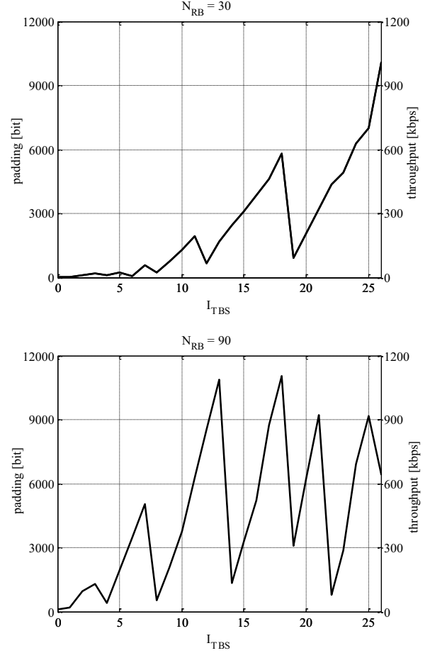
Figure 4. The size of padding and hidden channel capacity as a function of MCS ( I_{TBS} ) and available resources ( N_{RB} = \{30, 90\} ) for L_{IP} = 1\,500 bytes
