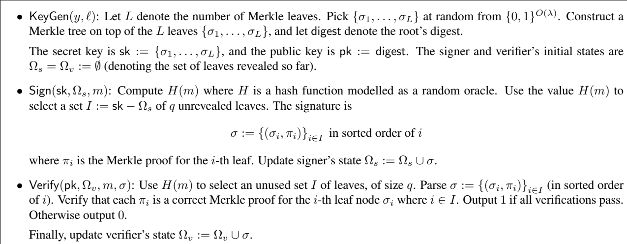
Figure 4: An FPS signature scheme.
