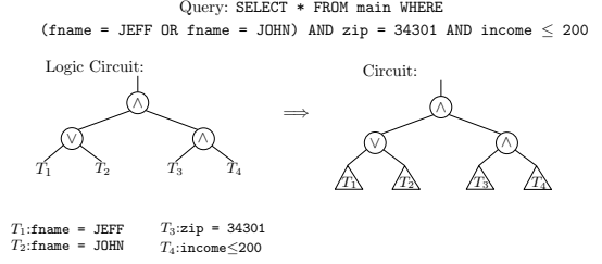
Figure 3. High level circuit representation of a query.
