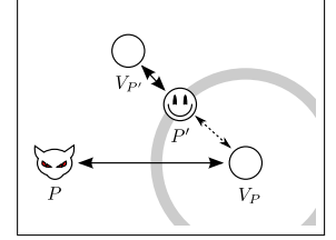
Figure 6. Scenario with multiple prover/verifier pairs, where V_x only accepts sessions from x . Even in this case, Distance Hijacking may be possible.
