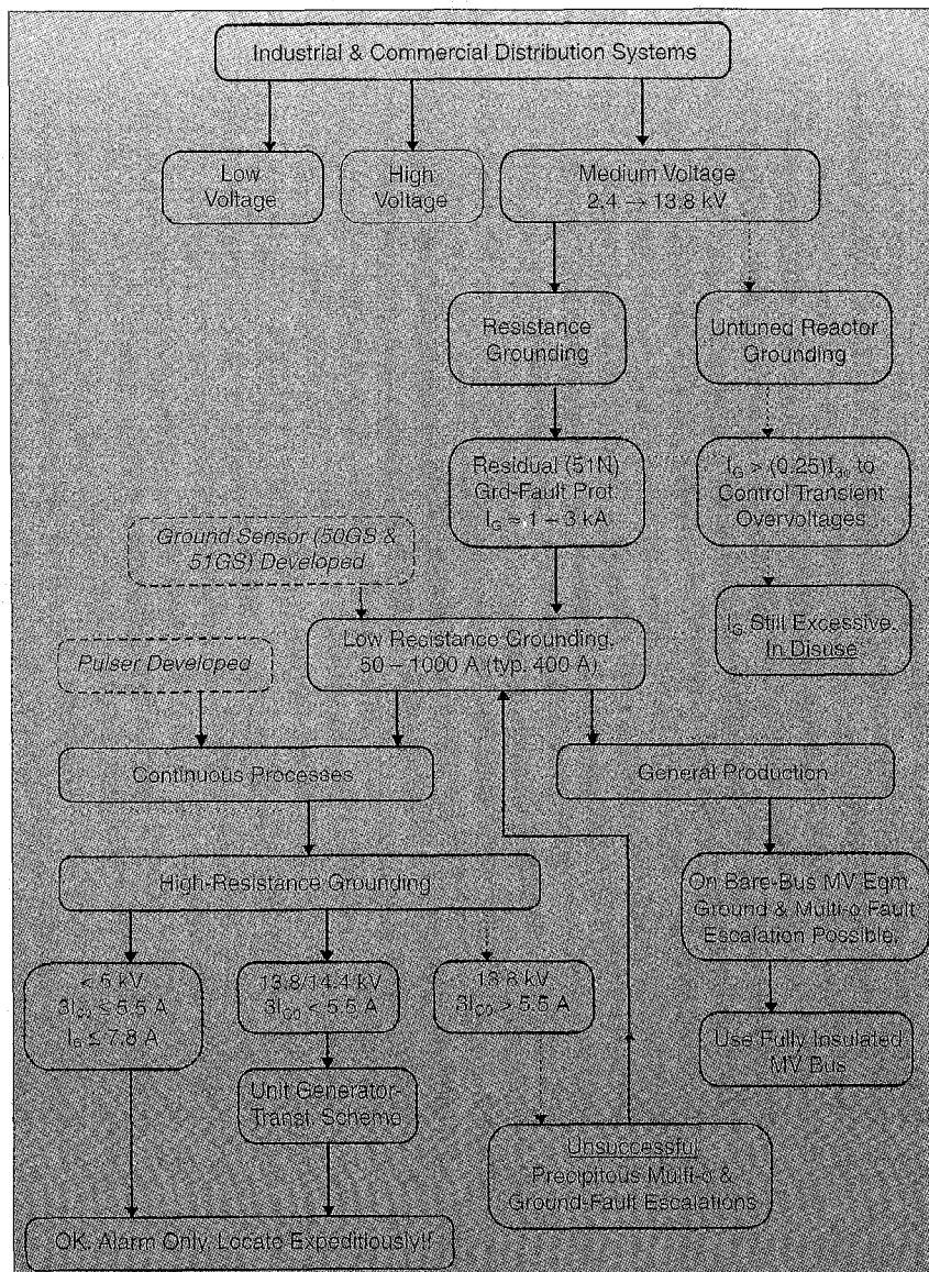
Fig. 3. Evolution of medium voltage neutral grounding practices in industry.
