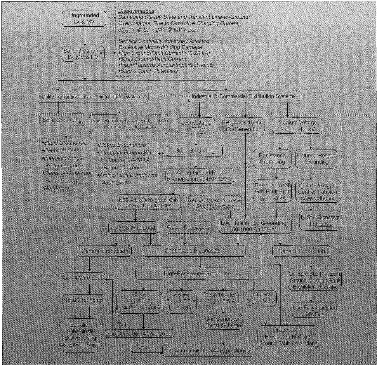
Fig. 4. Evolution of neutral grounding practices in the electrical industry.
