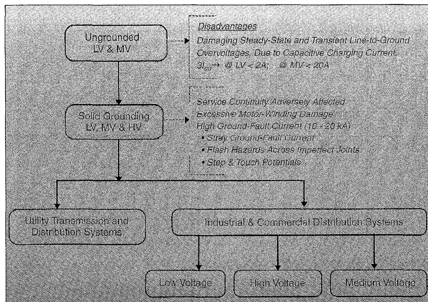
Fig. 1. Evolution of the early neutral grounding practices in the electrical industry.
