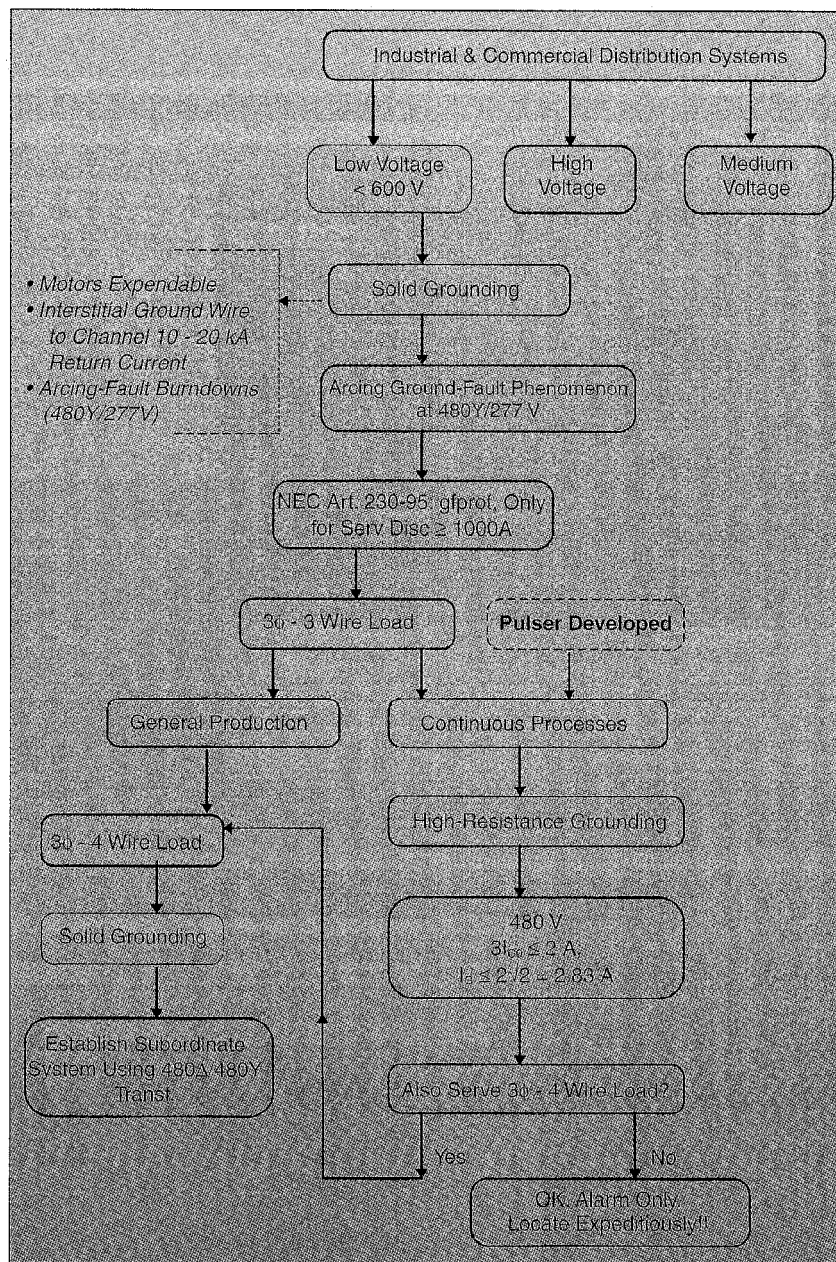
Fig. 2. Evolution of low-voltage neutral grounding practices in industry.
