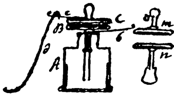
Figure 7: Volta's sketch of the "condensing electroscope," March, 1799 [1, 3:440].
