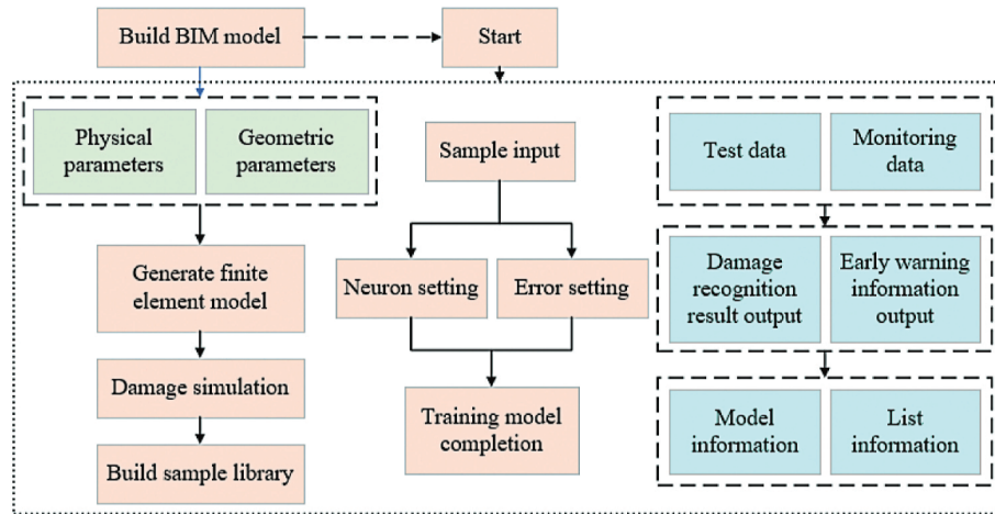
Fig. 7 AI-based BIM for intelligent structural damage recognition [70].
