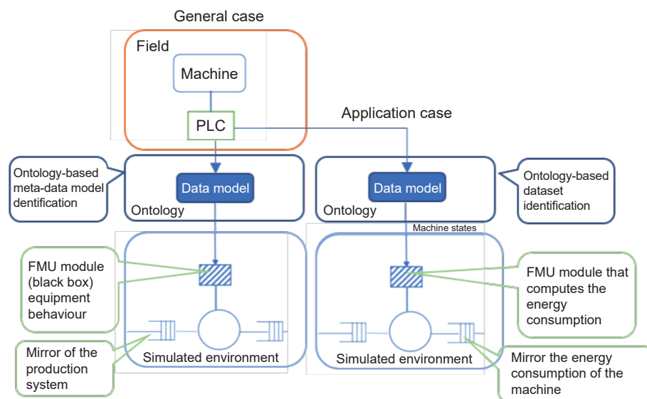
Fig. 1 FMUs in the application case (PLC: programmable logic controller) [46].
