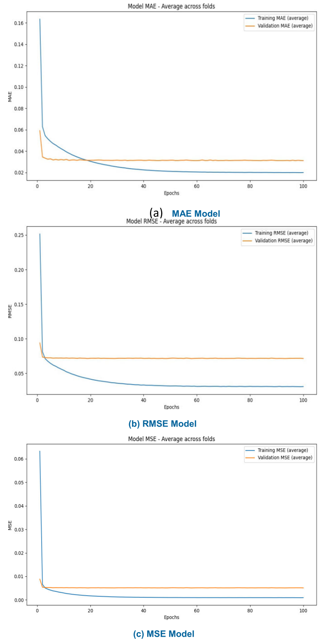
FIGURE 4. Performance metrics (MAE, RMSE and MSE) of the model.
