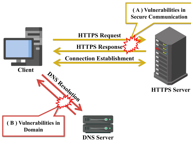
Fig. 6: Types of Attacks on HTTPS
