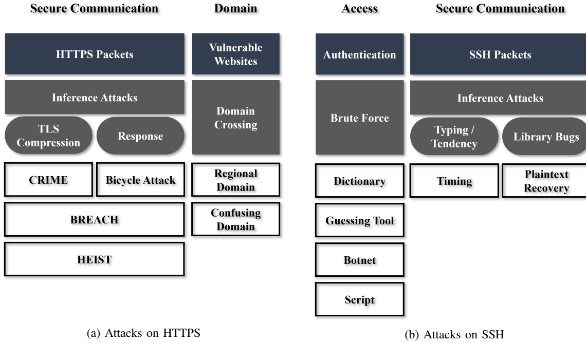
Fig. 5: Classification of attacks launched at the Application layer protocols. Targets are represented by navy boxes, strategies by gray boxes, and the names of publicly known attacks by white boxes. Wide boxes indicate attacks with multiple properties. Attacks on HTTPS are classified into secure communication and domain, and attacks on SSH are classified into access and secure communication.
