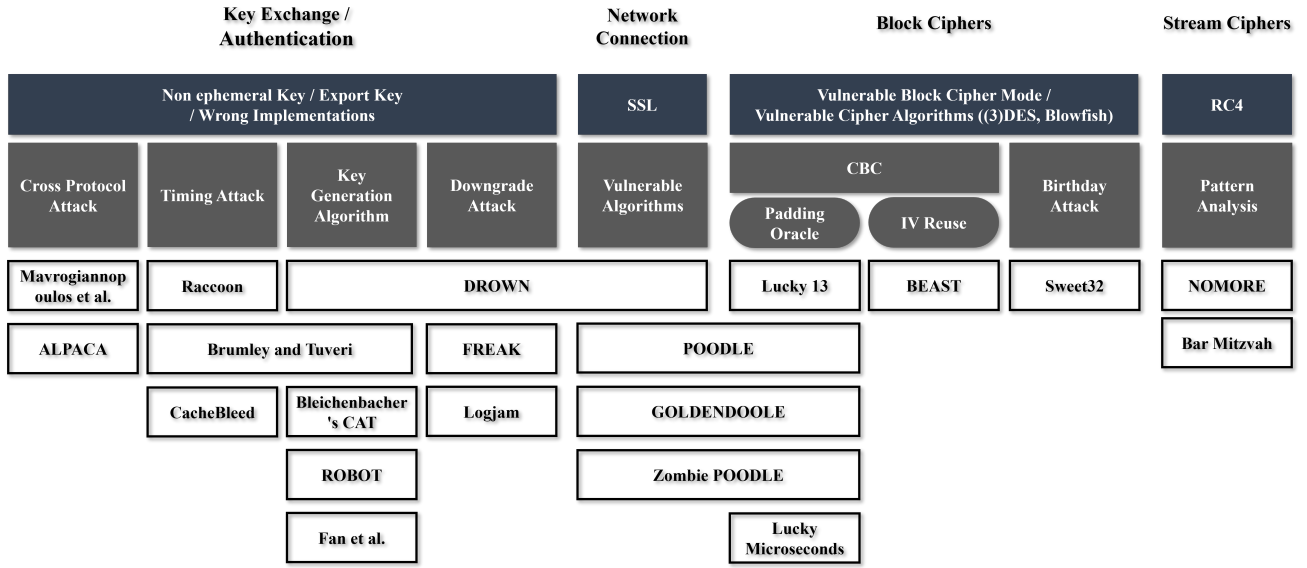
Fig. 3: Classification of vulnerabilities in the earlier versions of TLS. Targets are represented by navy boxes, strategies by gray boxes, and the names of publicly known attacks by white boxes. Wide boxes indicate attacks with multiple properties. These attacks are classified into four main cases: Key Exchange/Authentication, Network Connection, Block Cipher Algorithm, and Stream Cipher Algorithm.
