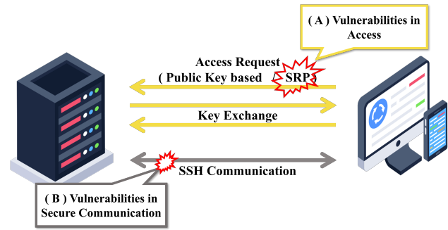
Fig. 7: Types of Attacks on SSH
