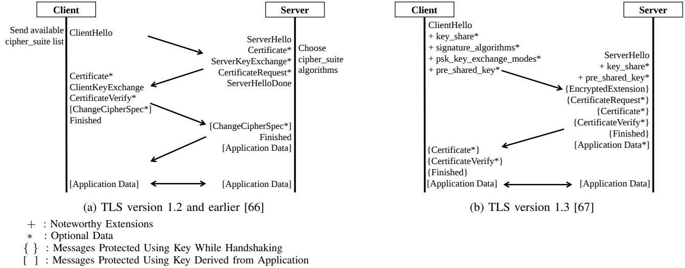
Fig. 2: Comparison of TLS Handshaking Protocols
