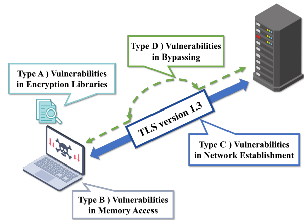
Fig. 4: Types of Attacks on TLS Version 1.3
