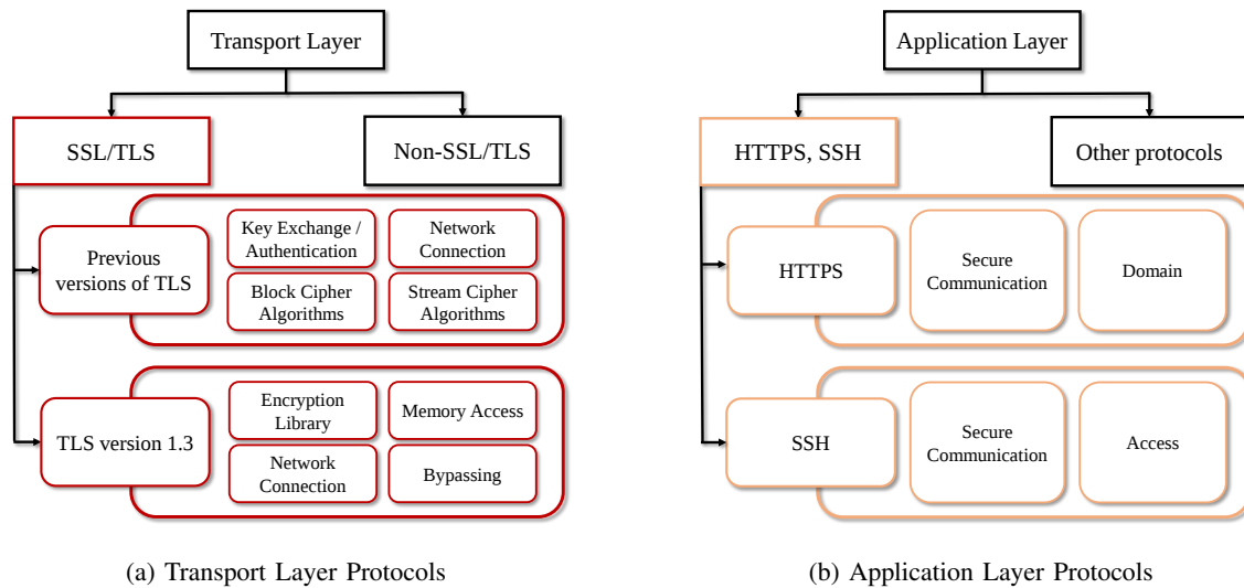
Fig. 1: Scope and objectives of our work. Red boxes in (a) and orange boxes in (b) represent topics covered in this paper.
