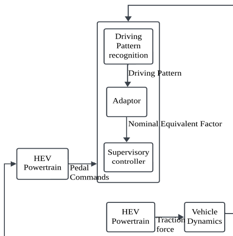
FIGURE 10. DPR approach to EMCS real-time adaptation.
