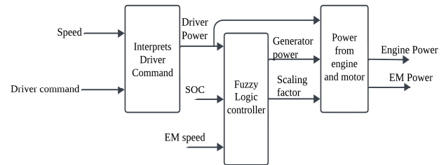
FIGURE 5. A simple fuzzy logic controller.
