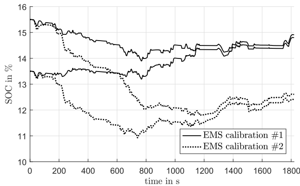
FIGURE 1. SOC trajectories of two EMS calibration variants for the same vehicle within the same driving cycle and two different start SOC.
