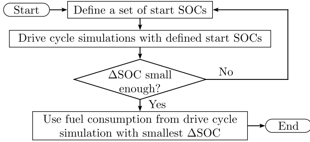
FIGURE 6. Flowchart for Variation of Start SOC method.
