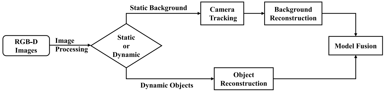
FIGURE 10. Overview of the dynamic indoor reconstruction pipeline. The first step is data acquisition, which is the same as in static 3D reconstruction. The second step is data preprocessing, which involves not only denoising the raw image data but also separating the dynamic objects from the scene. Then, camera tracking is performed using the static background information to align the current frame data with the previous frame or model, finding the correspondences between them and reconstructing the static background. Meanwhile, the dynamic objects are reconstructed separately. Finally, the dynamic objects and static background are merged to complete the reconstruction of the entire scene.
