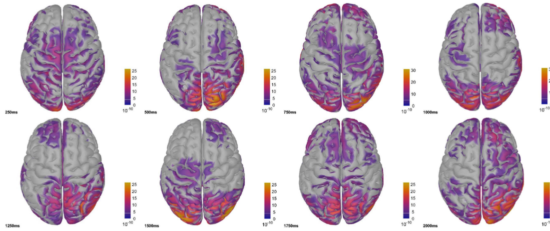
Fig. 8. The brain source localization analysis of one representative subject S9.
