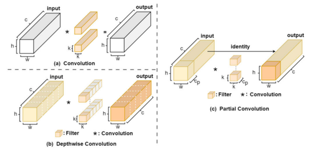
FIGURE 5. Comparison of ordinary convolution, DWConv, and PConv convolution: (a) Structural diagram of ordinary convolution, (b) Structural diagram of DWConv convolution, (c) Structural diagram of PConv convolution.
