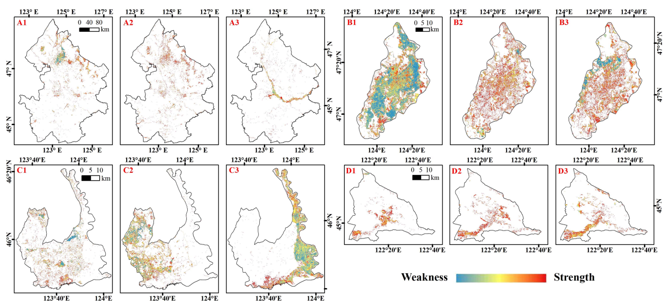
Fig. 8. CI of wetland plant communities from 2016 to 2022. (a1)–(a3) Results of P.a. , T.o. , and C.m. of western Songnen Plain. (b1)–(b3) Results of P.a. , T.o. , and S.t. of Zhalong Nature Reserve. (c1)–(c3) Results of P.a. , S.g. , and C.m. of Momoge Nature Reserve. (d1)–(d3) Results of P.a. , T.o. , and S.t. of Xianghai Nature Reserve.
