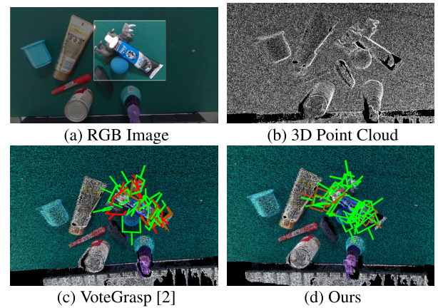
FIGURE 7. An illustrative example showcasing the performance contrast between our proposed method and the baseline approach. In this scenario, the highlighted objects are closely clustered together, making it challenging for baseline methods to generate high-quality grasps due to the proximity and occlusion. Our method, however, adeptly leverages fusion of appearance and geometry information to provide reliable grasps even in complex scenarios, demonstrating its superior performance in handling close proximity and occlusion challenges.
