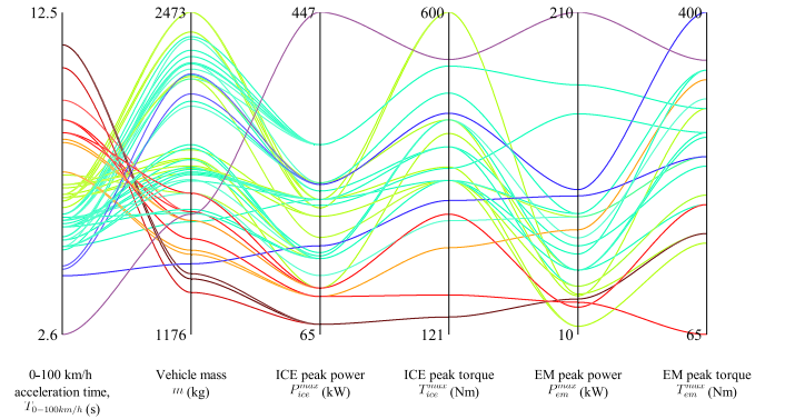
Fig. 2. Main specifications of hybrid vehicles from the database. Note: ICE = internal combustion engine; EM = electric motor.
