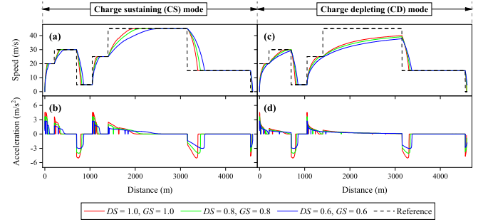
Fig. 5. Artificial driving cycle with the response of the MFC model: (a)-(b) CS mode; (c)-(d) CD mode.
