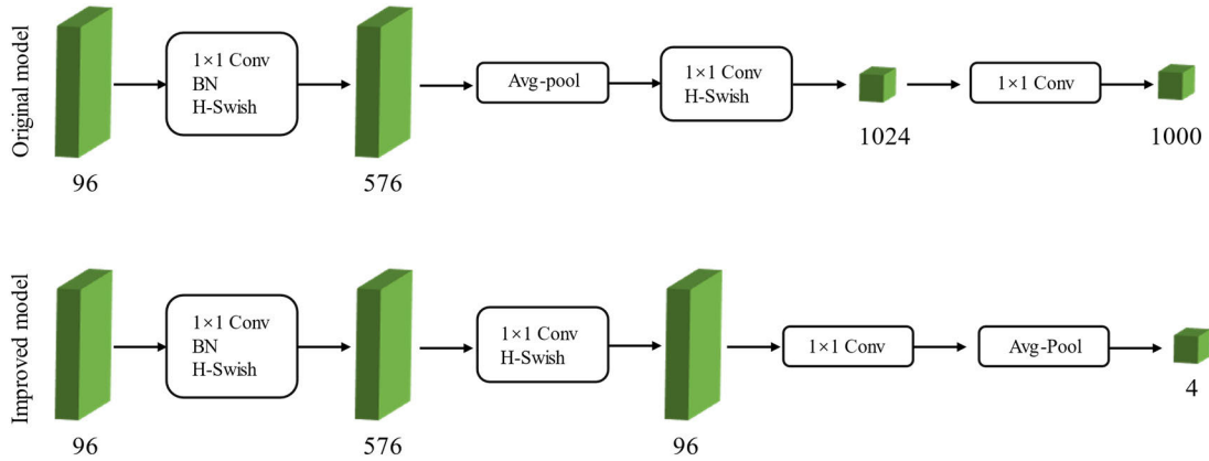
FIGURE 2. Network structure of improved model classification layer.
