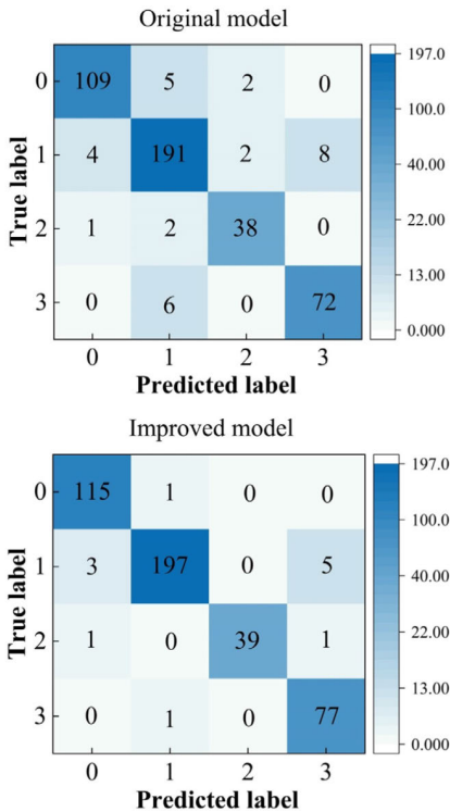
FIGURE 8. Confusion matrix.
