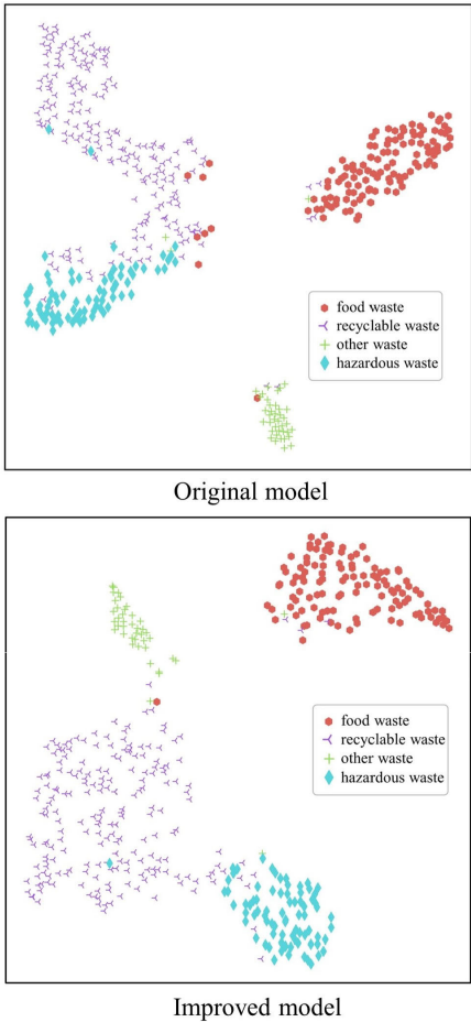
FIGURE 9. Visualization plots of t-SNE downscaling.
