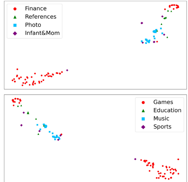
FIGURE 5. App node embeddings Visualization: Distinct separation of categories in the embedding space by MP-GT model.
