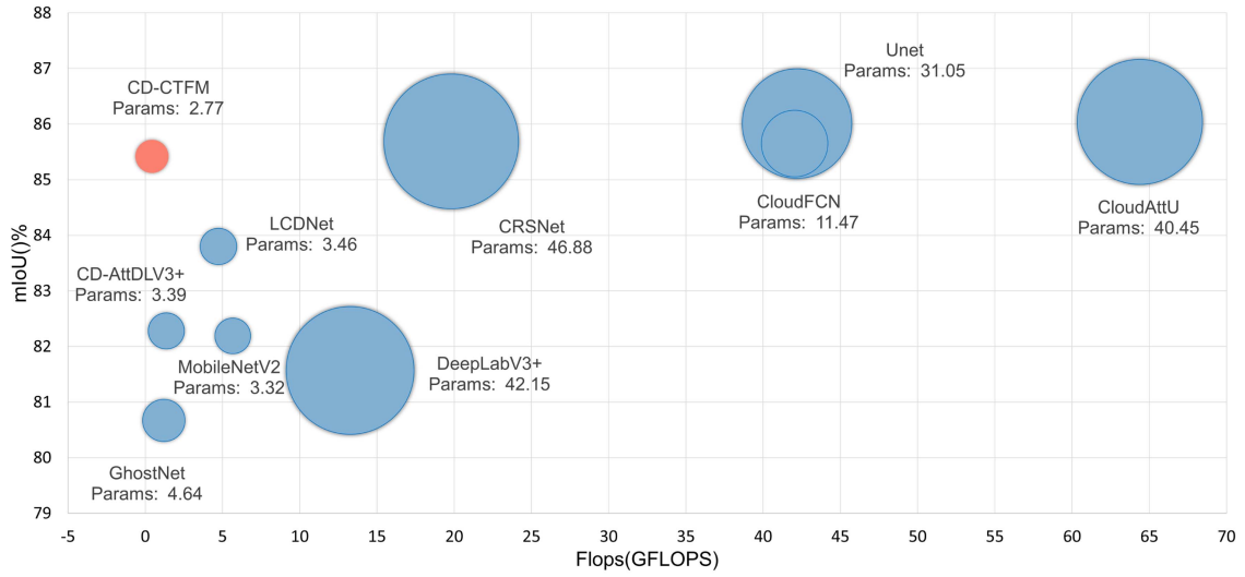
Fig. 8. mIoU performance, GFLOPS, and parameters of cloud detection models on 38-Cloud dataset. x-axis is the GFLOPS, y-axis is the mIoU, and the size of bubble represents the parameters. Here, CD-CTFM is compared with UNet, DeepLabV3+, CloudFCN, CloudAttU, CRSNet, MobileNetV2, GhostNet, CD-AttDLV3+, and LCDNet.
