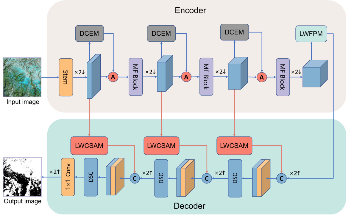
Fig. 1. Overall framework of CD-CTFM. The encoder contains a lightweight backbone and LWFPM while the decoder is based on DSC. LWCSAM filters information propagated through the skip connections.
