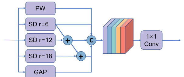
Fig. 5. Structure of LWFPM.
