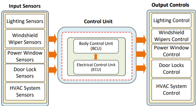
FIGURE 13. Basic configuration of BCU using input sensors and output controls.
