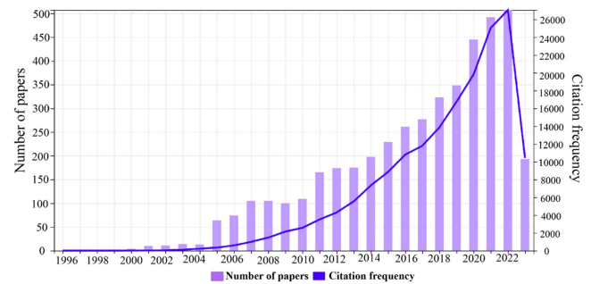
Fig. 11. Frequency of citations to articles on carbon emissions and the number of published papers.
