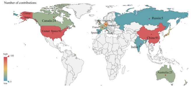
Fig. 10. Contribution of different countries in the field of carbon emissions for the two years 2020–2023.
