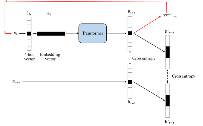
FIGURE 5. Sketch of the TrAISformer architecture: each AIS observation \mathbf{x}_t is discretized into a “four-hot” vector \mathbf{h}_t (for visualization purposes, we illustrate a one-hot vector instead of a “four-hot” vector for \mathbf{h}_t ). Subsequently, each \mathbf{h}_t is paired with a high dimensional real-valued embedding vector \mathbf{e}_t . The sequence of embeddings the \mathbf{e}_{0:t} will be fed into a transformer network to predict p_{t+1} \triangleq p(\mathbf{h}_{t+1}|\mathbf{e}_{0:t}) . During the training phase, the model is optimized to minimize the cross-entropy loss between the true value \mathbf{h}_{t+1} and p_{t+1} . To enhance prediction accuracy, we introduce a “multi-resolution” loss. This involves calculating the cross-entropy at different spatial resolutions of \mathbf{h}_{t+1} . In the forecasting phase, we generate vessel positions recursively. We sample \mathbf{h}_{t+1}^{pred} from p_{t+1} , calculate the “pseudo-inverse” of it to derive \mathbf{x}_{t+1}^{pred} . The predicted \mathbf{x}_{t+1}^{pred} is fed back into the network to sample the next position (as shown by the red path in the diagram). This iterative process continues until we reach the desired prediction horizon L .
