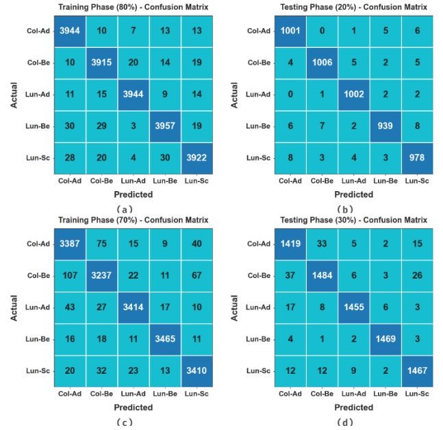
FIGURE 4. (a-b) Confusion matrices of IWSACAE-LCCD method 80:20 of TRS/TSS and (c-d) 70:30 of TRS/TSS.
