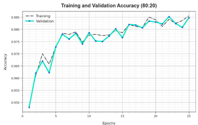
FIGURE 7. Accuracy curve of IWSACAE-LCCD approach at 80:20 of TRS/TSS.
