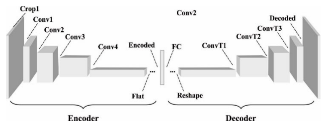
FIGURE 2. CAE structure.
