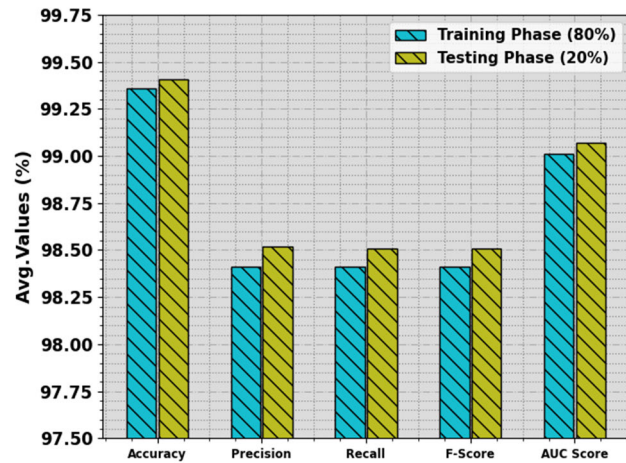
FIGURE 5. Average of IWSACAE-LCCD approach at 80:20 of TRS/TSS.
