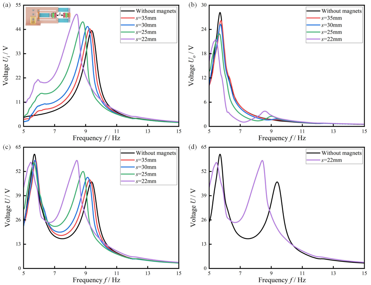
FIGURE 7. The open-circuit output voltage under changing the magnetic spacing: (a) The output voltage of the inner beam; (b) The output voltage of outer beams; (c) The total output voltage of the inner and outer beams; (d) The comparison between the proposed PVEH under the magnetic spacing is 22 mm and the PVEH without magnets.
