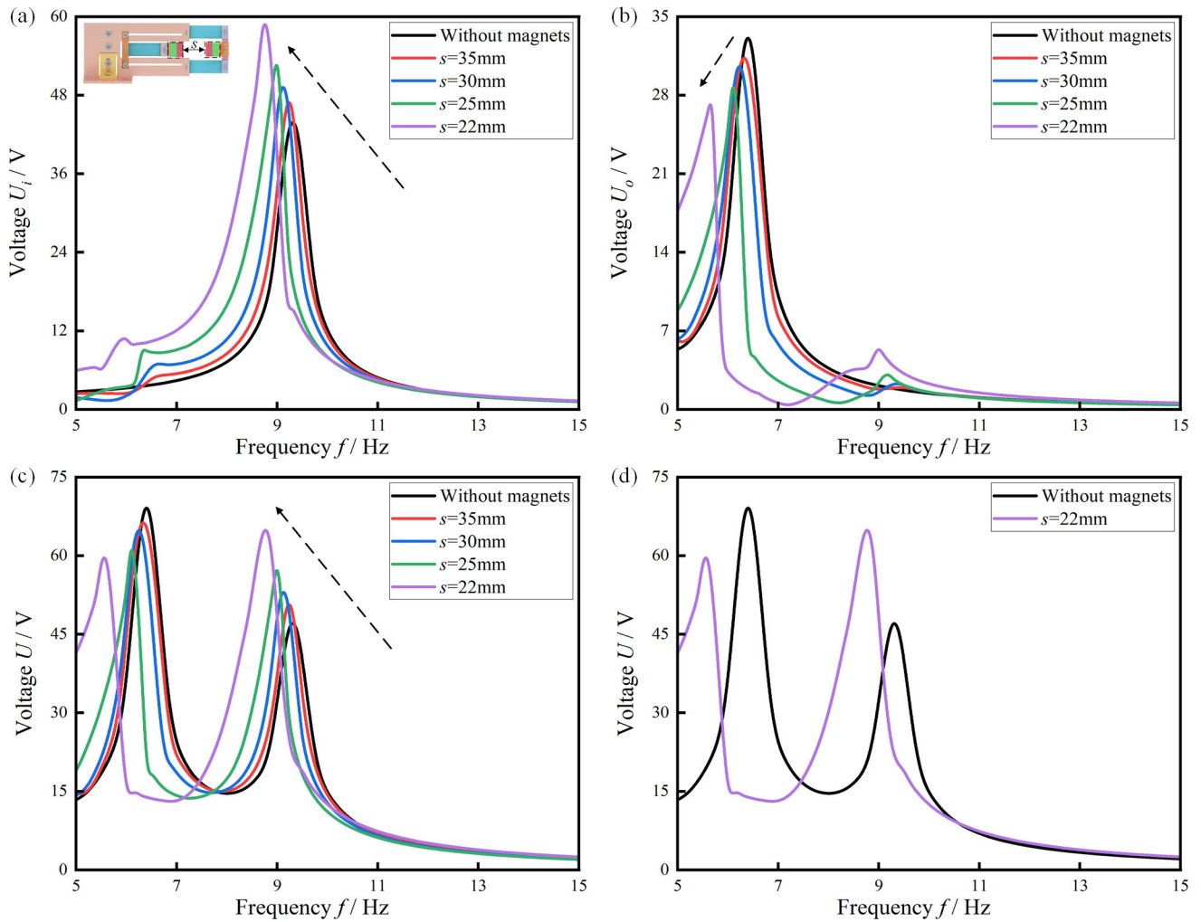
FIGURE 4. The simulation results of changing the magnet spacing: (a) The output voltage of the inner beam; (b) The output voltage of outer beams; (c) The total output voltage of the inner and outer beams; (d) The comparison between the proposed PVEH under the magnetic spacing is 22 mm and the PVEH without magnets.
