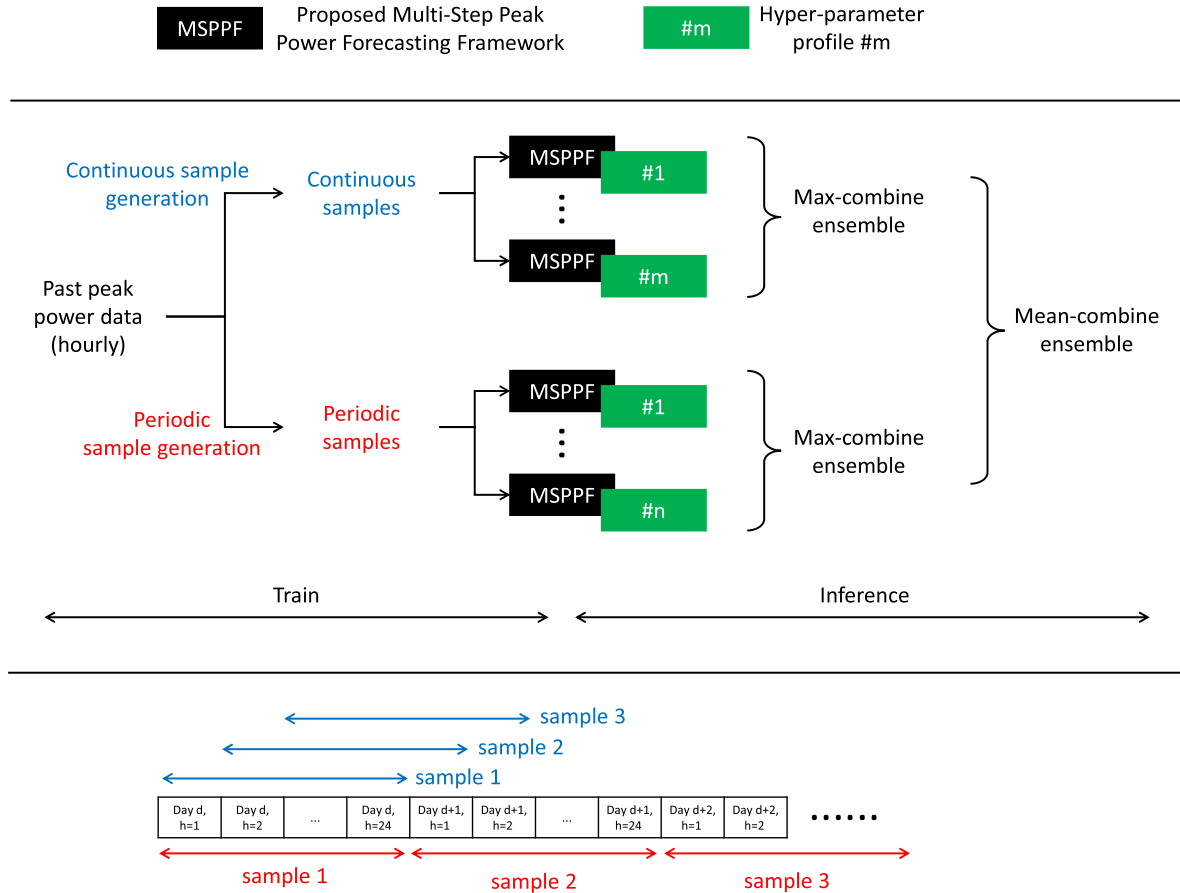
FIGURE 3. The proposed two sample construction methods, i.e., continuous sampling and periodic sampling, and two-level ensemble strategies, i.e., lower-level max-combine and upper-level mean-combine ensemble.
