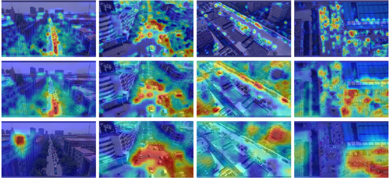
FIGURE 18. The attention of different detection heads to the small objects.
