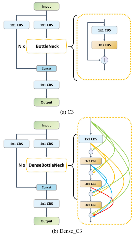
FIGURE 7. The structure of the C3 and Dense_C3. The (a) is the C3 structure, and the (b) is the Dense_C3 structure with dense connection mechanism.
