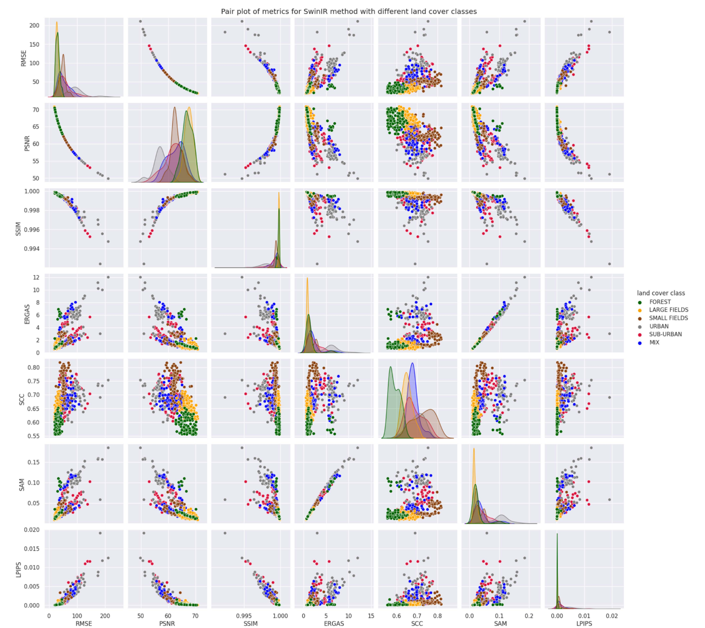
Fig. 24. Pair plot for metrics for SwinIR.
