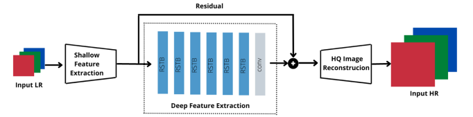
Fig. 4. Scheme of the SwinIR network architecture with Residual Swin Transformer Block (RSTB).
