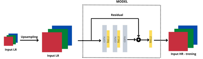
Fig. 3. Scheme of the SRCNN network architecture with changes.
