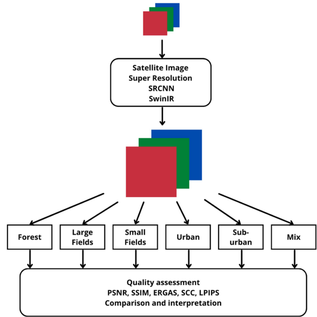
Fig. 1. Simplify flowchart of the experiment.
