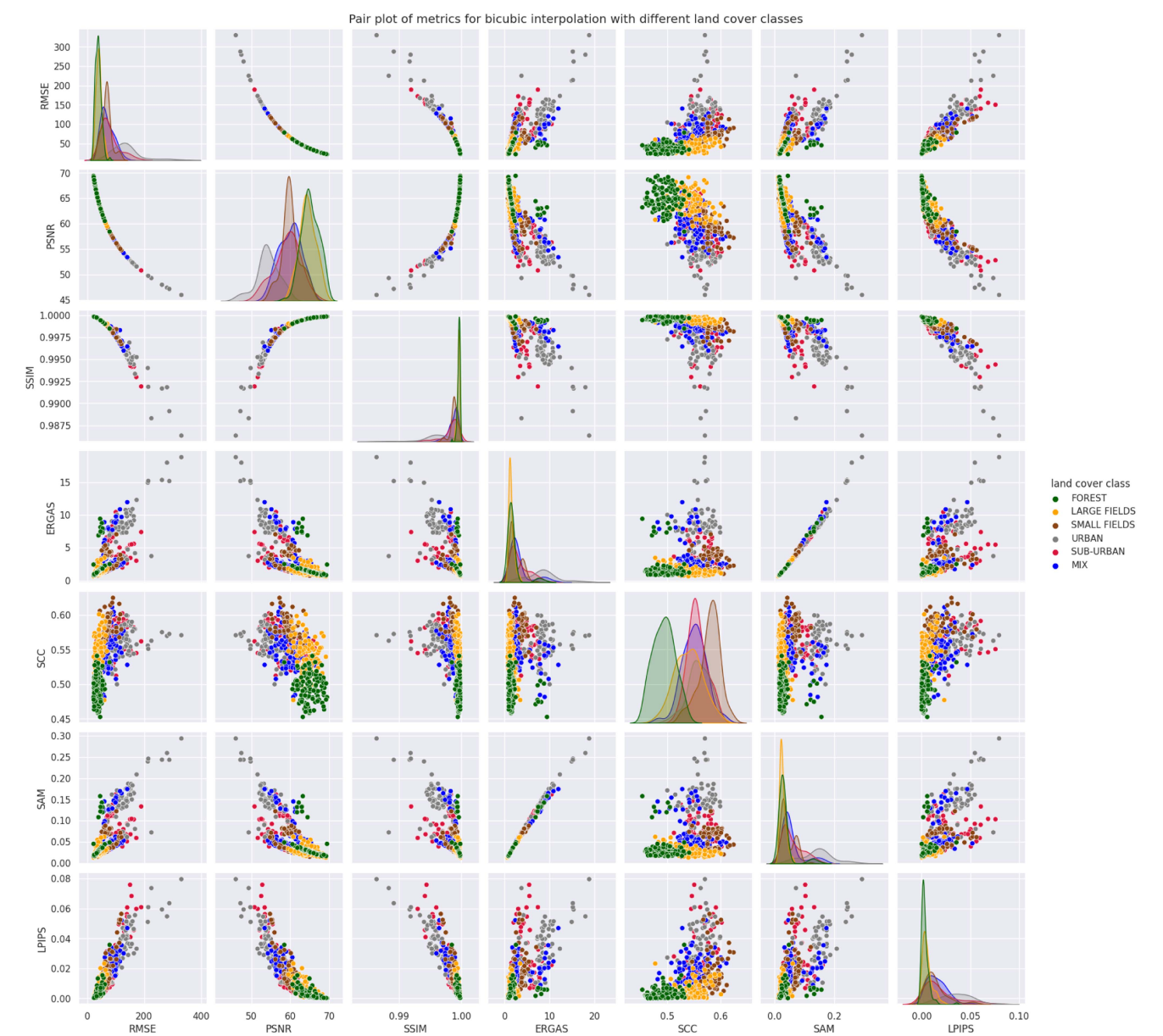
Fig. 22. Pair plot for metrics for bicubic interpolation.
