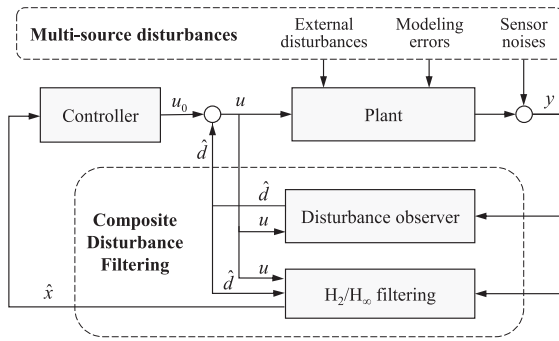
FIGURE 4. Composite DO+ H_2/H_\infty filtering scheme.
