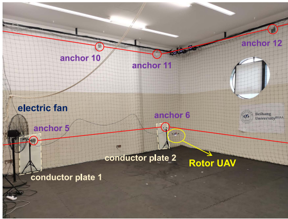
FIGURE 7. Flight test of UAV indoor localization.
