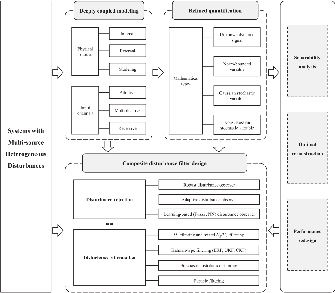
FIGURE 2. Principle of the CDF scheme.
