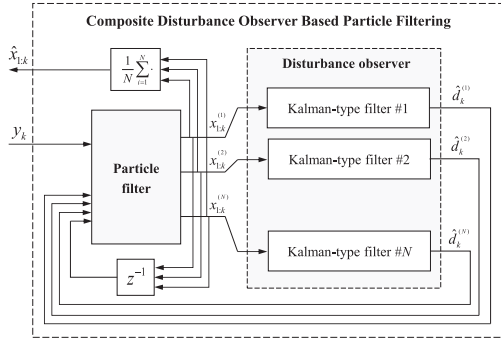
FIGURE 5. Composite DO+PF approach.
