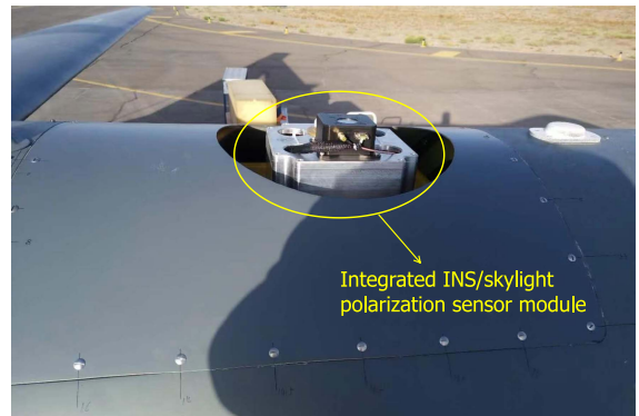
FIGURE 9. Application to "CH"-series UAV.
