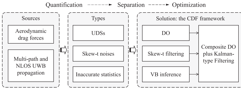
FIGURE 6. Separation of heterogeneous disturbances in UAV localization.
