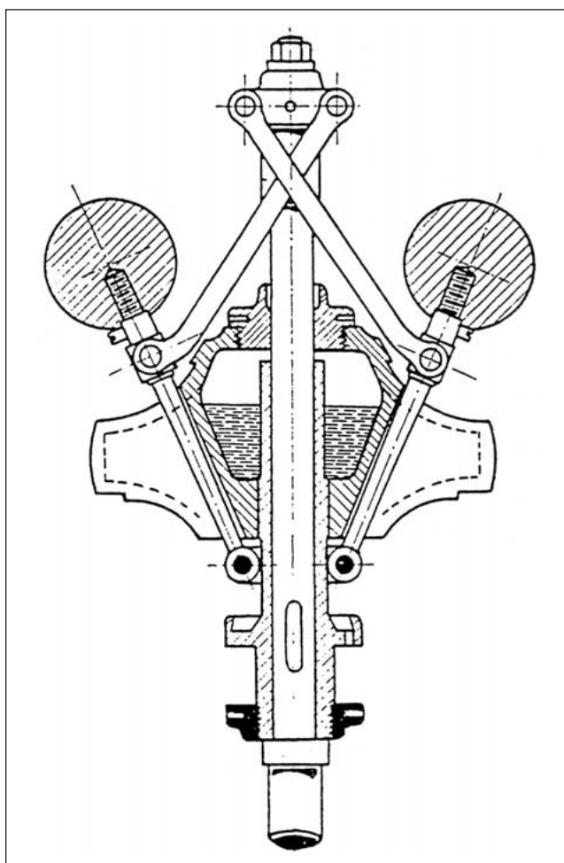
Figure 5. A nonstatic parabolic regulator, 1880 (from [11], [22]).
