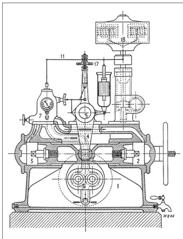
Figure 9. Universal governor of Escher Wyss, Zurich, 1906 (from [29]).
