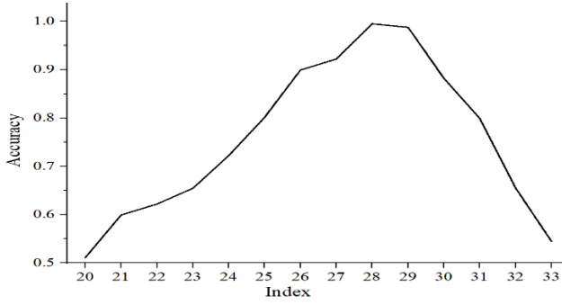
FIGURE 4. Classification accuracy corresponding to different n values.
