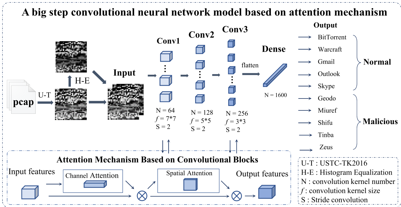
FIGURE 1. Flowchart of network traffic classification.
