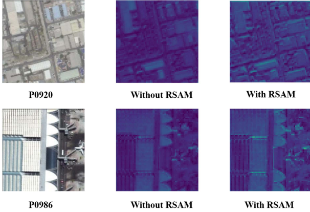
Fig. 9. Comparison of feature map visualization with/without RSAM.
