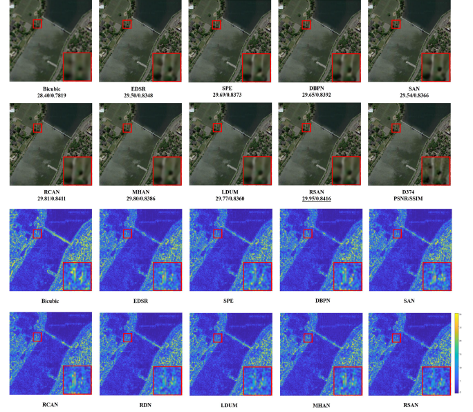
Fig. 3. Visual results with \times 4 of the RSSCN7 dataset. The final two rows of images show the error map.
