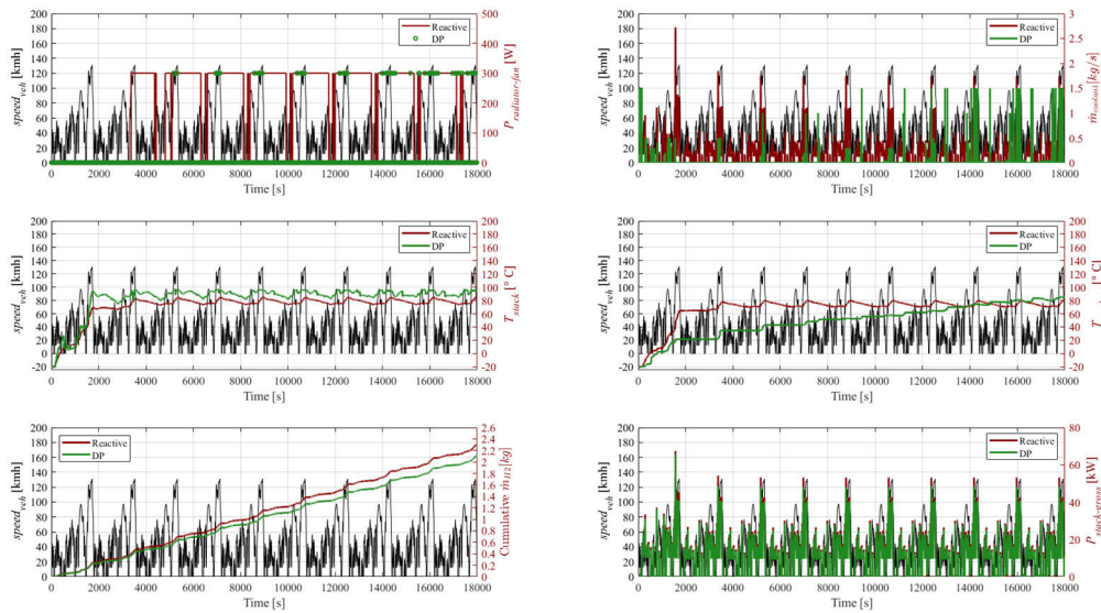
FIGURE 12. Time series of control and state variables for the FCEV simulated at -20^{\circ}\text{C} ambient temperature being controlled by both DP and the baseline reactive control strategy from Advisor in WLTCx10.
