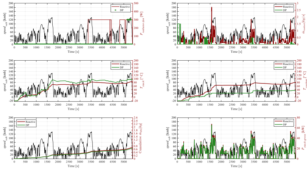
FIGURE 11. Time series of control and state variables for the FCEV simulated at -20^{\circ}\text{C} ambient temperature being controlled by both DP and the baseline reactive control strategy from Advisor in WLTCx3.
