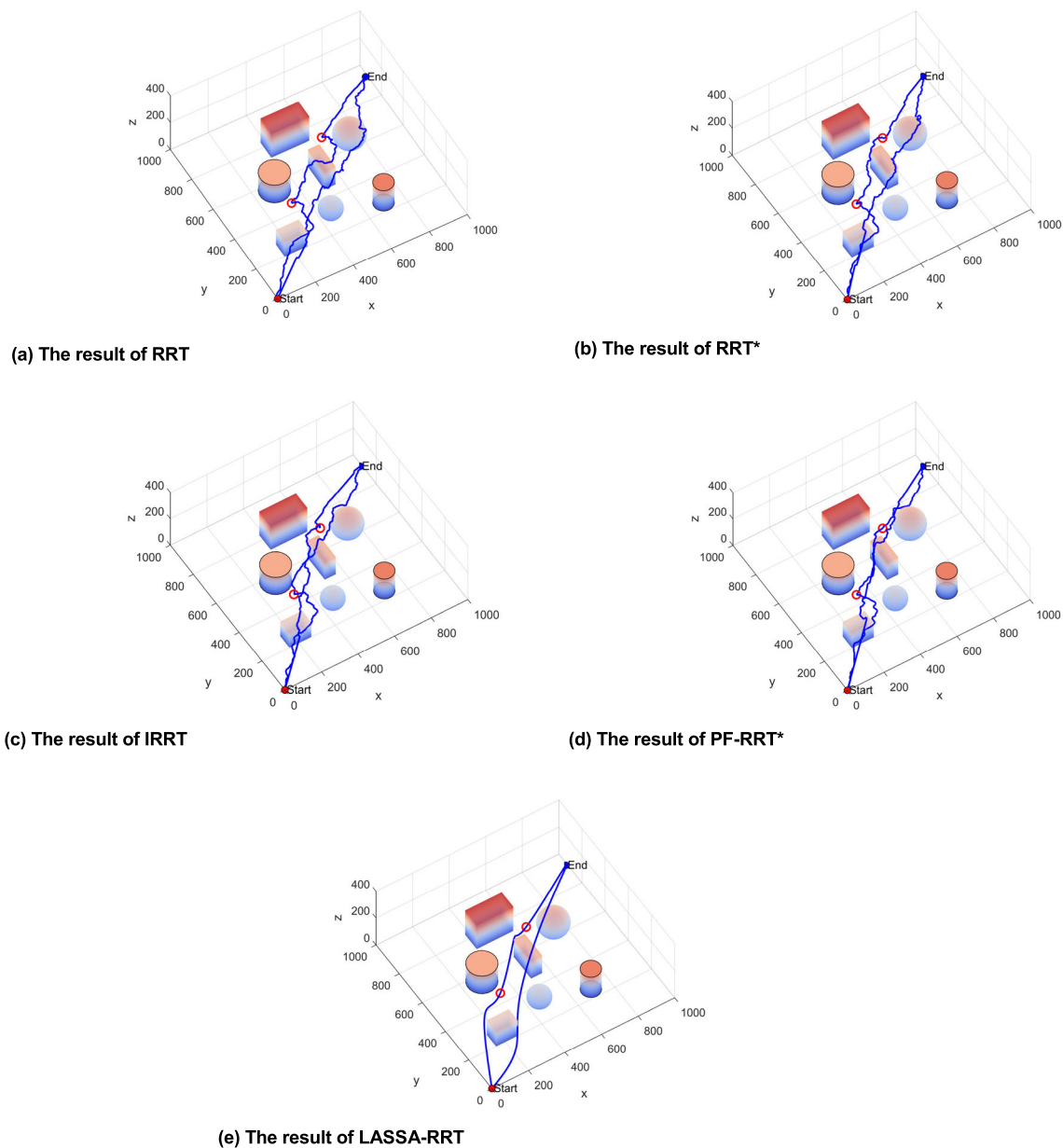
FIGURE 13. Running results of each algorithm under scenario A.
