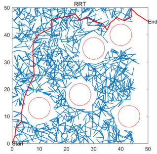
FIGURE 3. The result of RRT algorithm.
