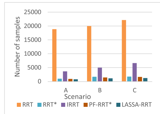
(d) Comparison results of number of samples
