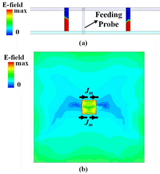
FIGURE 7. Complex E-field magnitude distribution on the (a) the blind via and (b) the patch and the ground plane.
