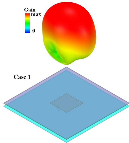
FIGURE 4. Simulated 3-D radiation pattern of Case 1.
