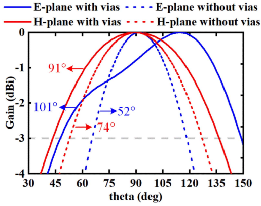
FIGURE 6. Comparison of E- and H-planes normalized radiation pattern of with blind via (Case 2) and without blind via (Case 1).
