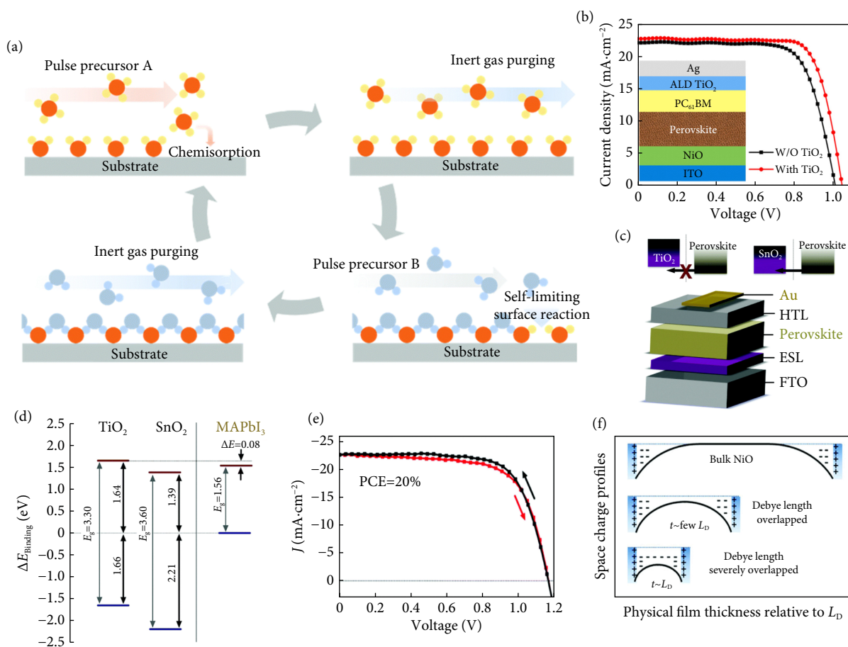
Fig. 5 ALD for CTLs. (a) Schematic illustration of the ALD process (reprinted with permission from ref. [45], © 2019 The Royal Society of Chemistry). (b) Device structure and J - V curve of PSC using ALD- \text{TiO}_2 as ETL (reprinted with permission from ref. [65], © 2018 American Chemical Society). (c and d) Schematic conduction band diagram of the perovskite films and the electron selective layers, \text{TiO}_2 and \text{SnO}_2 for \text{MAPbI}_3 PSCs (reprinted with permission from ref. [69], © 2015 The Royal Society of Chemistry). (e) Current-voltage characteristics of the PSC using ALD- \text{SnO}_2 as ETL (reprinted with permission from ref. [70], © 2017 The Royal Society of Chemistry). (f) Schematic images of physical film thickness relative to the Debye length versus space charge profiles (reprinted with permission from ref. [72], © 2016 The Royal Society of Chemistry).
