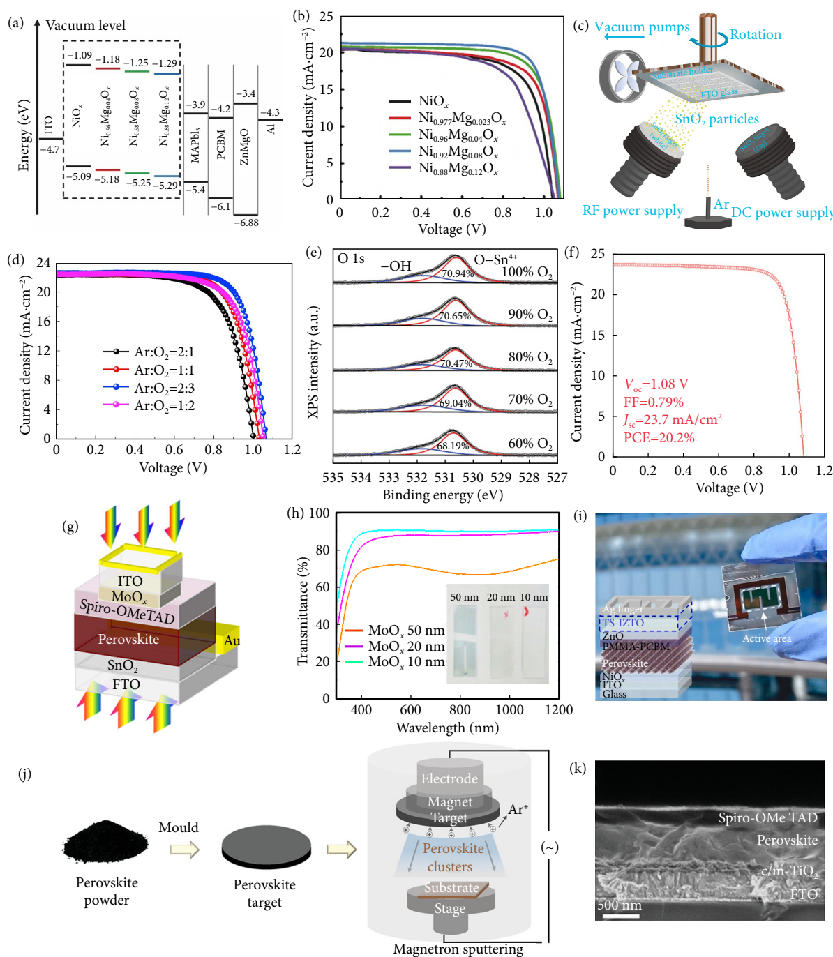
Fig. 7 Applications of magnetron sputtering for fabricating PSCs. (a and b) Energy band diagram (a) and current-voltage characteristics (b) of sputtered MgO doped \text{NiO}_x as ETL (reprinted with permission from ref. [81], © 2017 The Authors). (c) Schematic illustration of \text{SnO}_2 deposition process of DC/RF magnetron sputtering. (d) J - V curves of PSC based on sputtered \text{SnO}_2 film with different Ar/ \text{O}_2 ratio. (e and f) Reprinted with permission from ref. [82], © 2019 International Solar Energy Society. (e) XPS O 1s core level of the \text{SnO}_2 films deposited with different oxygen ratio. (f) J - V curve of the champion device based on the sputtered \text{SnO}_2 ETL and \text{MAPbI}_3 perovskite film. (e and f) Reprinted with permission from ref. [83], © 2019 The Authors. (g) Schematic illustration of the semi-transparent PSC with two illumination direction. (h) Transmittance of different thicknesses of \text{MoO}_x buffer layers. (g and h) Reprinted with permission from ref. [74], © 2017 Elsevier Ltd. (i) Photograph and schematic device structure of semi-transparent PSC with ITO anode and IZTO top cathode (reprinted with permission from ref. [85], © 2020 Elsevier Ltd). (j) Scheme of the perovskite layer preparation process via sputtering. (k) Cross-sectional SEM image of PSCs produced via magnetron sputtering. (j and k) Reprinted with permission from ref. [87], © 2021 The Authors.
