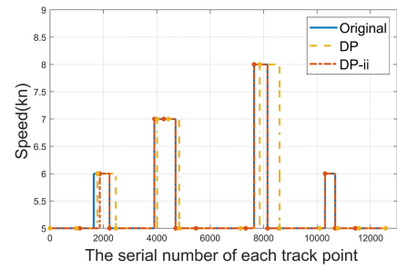
FIGURE 12. Comparison of the speeds in Case 2.
