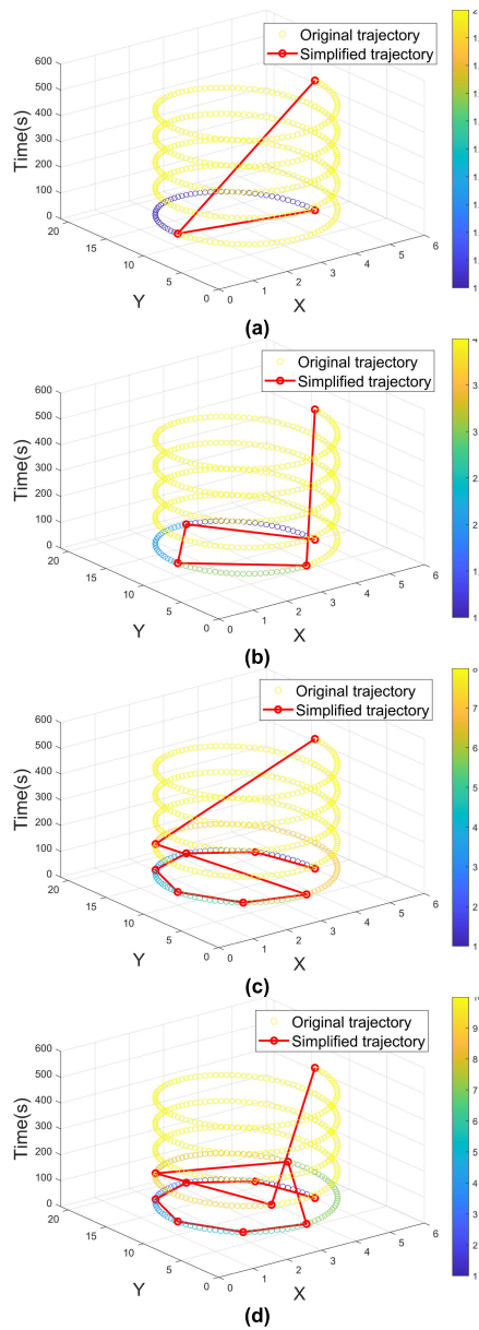
FIGURE 18. Case 4 trajectory compression process using the DP algorithm: compressions after (a) one, (b) two, (c) three, and (d) four layers. Note: the same color track points in the figure are in the same subset.
