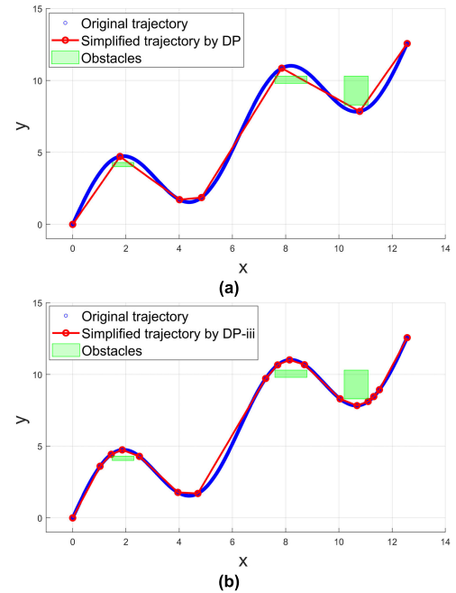
FIGURE 13. Compression results of the Case 3 trajectory using the (a) DP and (b) DP-iii algorithms.
