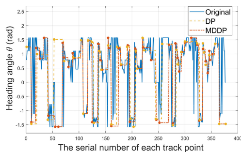
FIGURE 32. Comparison of heading angles of Case 7.
