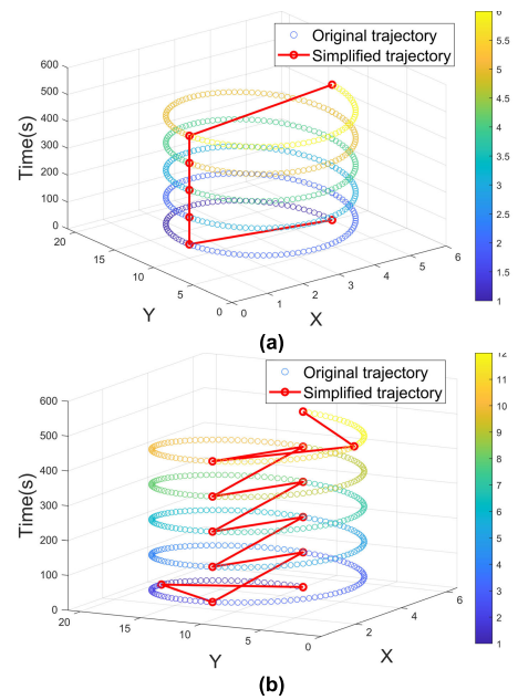
FIGURE 19. Case 4 trajectory compression process using the MPDP algorithm: compression after (a) one and (b) two layers. Note: the same color track points in the figure are in the same subset.
