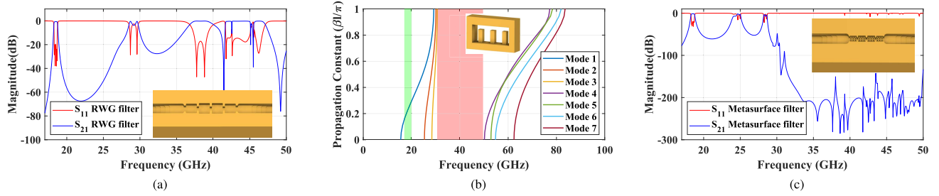
Fig. 2. Comparison of RWG filter and metasurface filter's frequency response. (a) Frequency response of a fourth-order RWG inline filter. (b) Propagation constant of the proposed metasurface transmission line. (c) Frequency response of the fourth-order metasurface inline filter.
