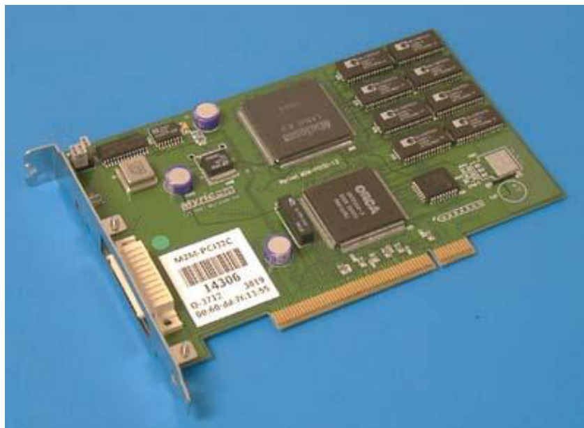
Figure 1: Myricom M2M-PCI32c network interface card. (Image credit: CSPi)
